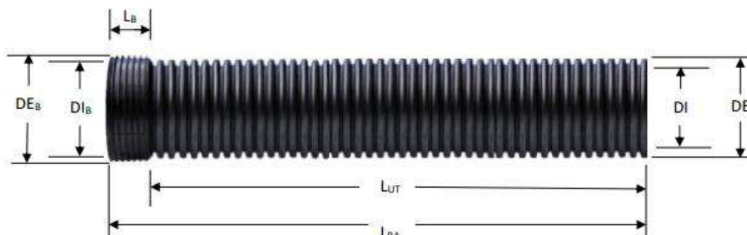
Figura 4 - Tubo KNTS Drain
